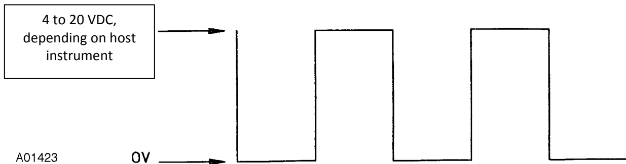
Figure 7. 61-12N-64P Output Voltage Waveform
